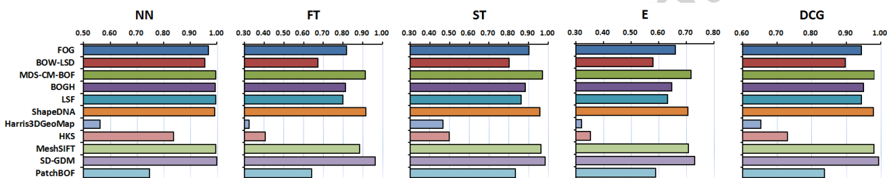
Figure 14: Bar charts of the retrieval accuracies of 11 methods evaluated on the whole database using five standard measures, respectively.
