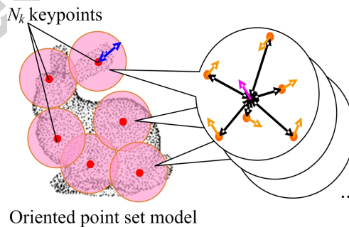
Figure 8: Localized Statistical Features (LSF).
